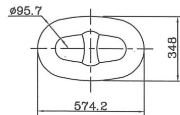
④ ENLARGED LINK
