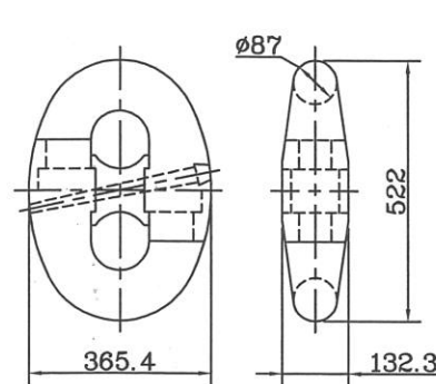
② KENTER SHACKLE
