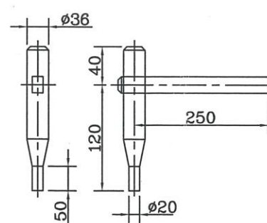
⑦ PIN PUNCH("A" TYPE)
