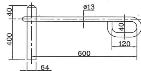
⑥ SHACKLE PUNCH
