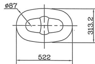
① ANCHOR SHACKLE
