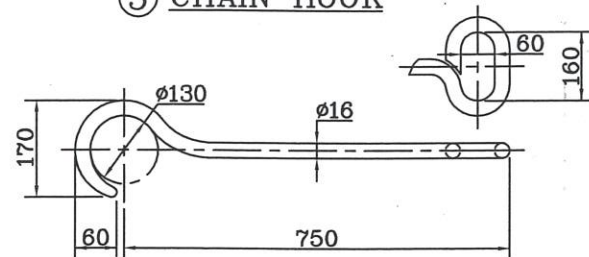
⑤ CHAIN HOOK
