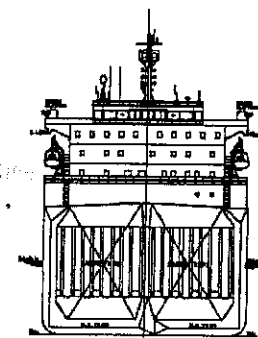
MIDSHIP SECTION
