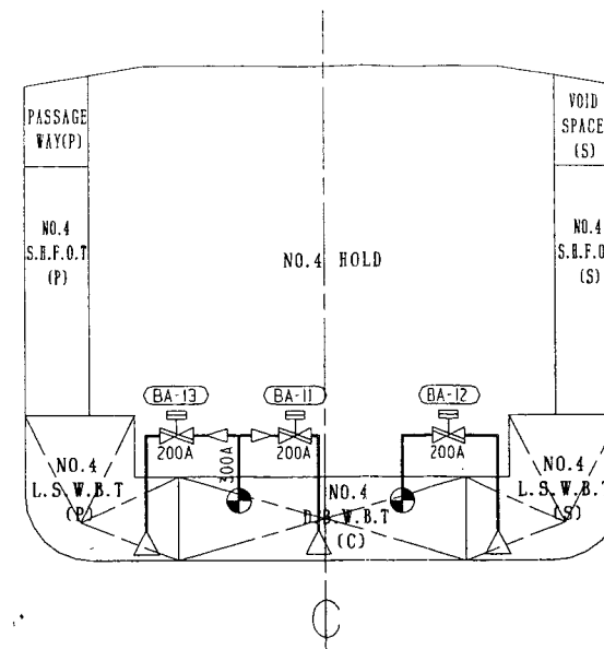
B-B SECTION
